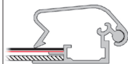
32 MM PROFILE
